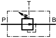
Hydraulic scheme
